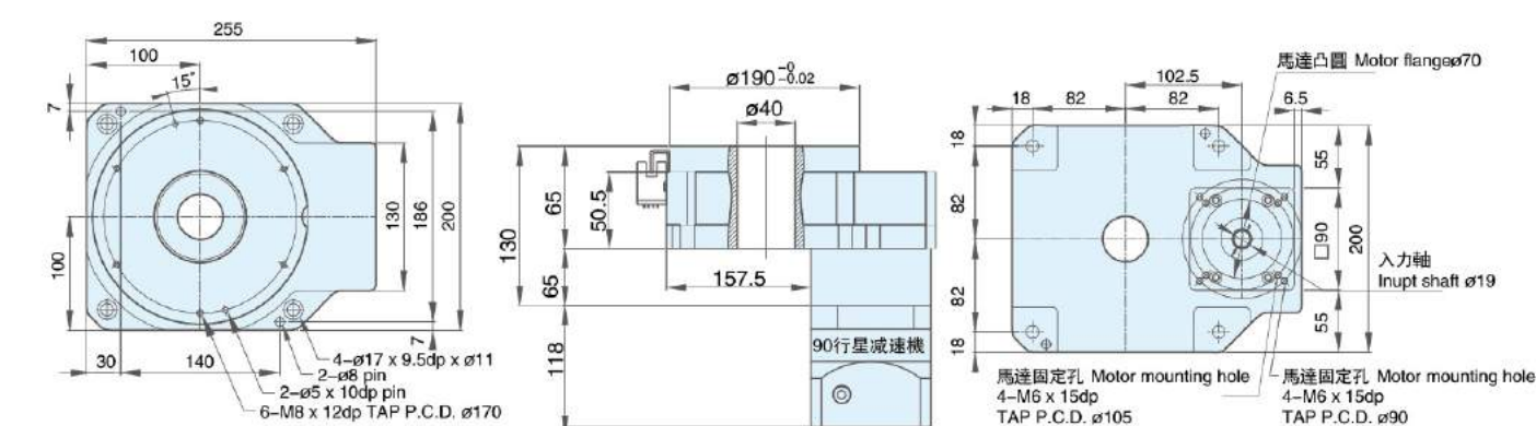
ZK 200P (附行星減速機速比 30,40,50)
