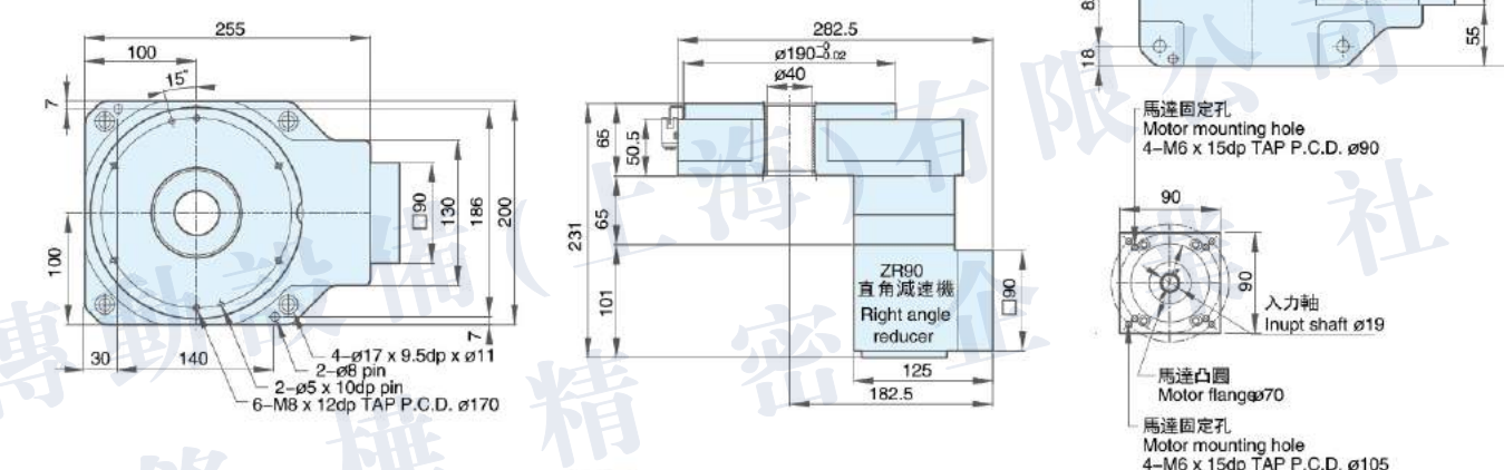
ZK 200P (附行星減速機速比 30,40,50)
